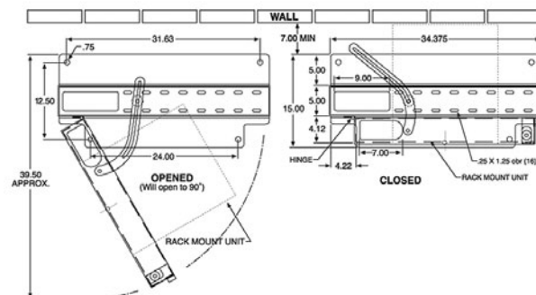
Swing Racks
